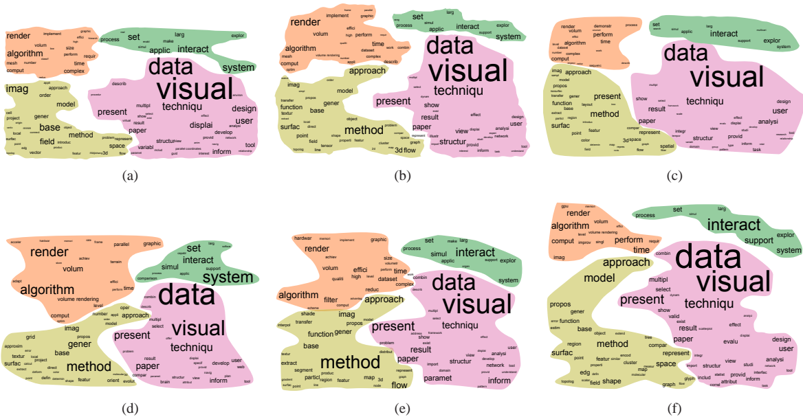
Figure 6: (a)-(c) semantic-preserving word clouds of IEEE Vis/InfoVis paper abstracts at 1999, 2005, and 2010; (d)-(f) semantic-preserving word clouds of EuroVis paper abstracts at 1999, 2005, and 2010.
